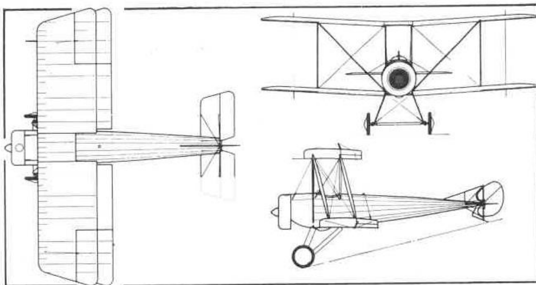
Grahame-White Type 20
